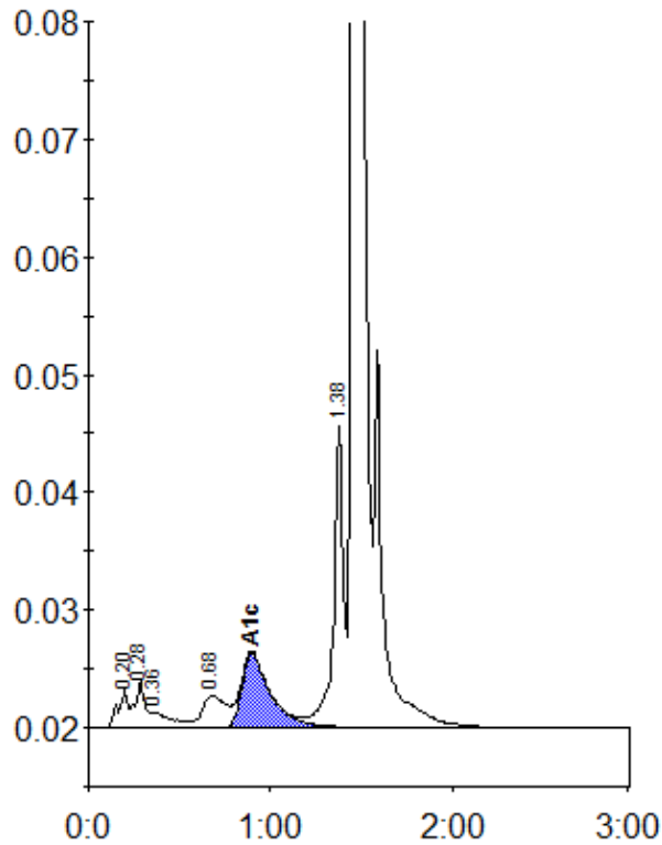
Peak table - ID: 10151476
